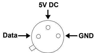
TO18 type SMT16030 with terminals towards viewer
